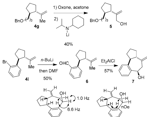
Scheme 3. Synthetic Applications
