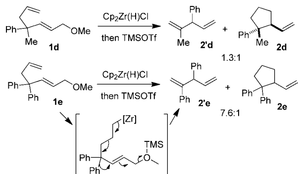
Scheme 1. Diene vs Vinylcyclopentane Formation
