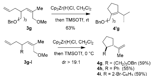
Scheme 2. Diastereoselective Synthesis of 2-Substituted Vinylcyclopentanes
