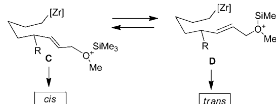
Figure 2. Diastereoselectivity rationale.
