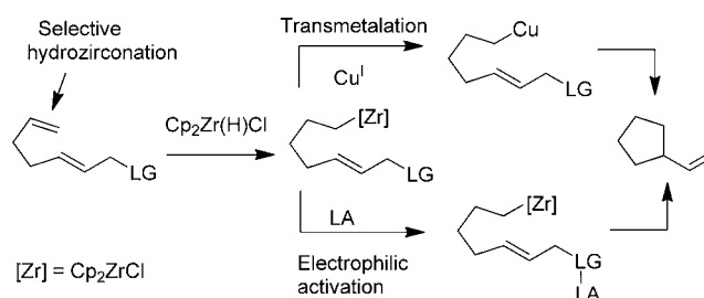
Figure 1. Approach toward vinylcyclopentanes.
